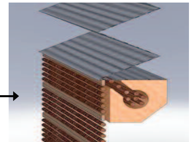
TriLight intermediate connecting rail detail view
